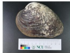
Lamprotula mansuyi
